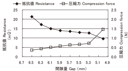
圧縮抵抗特性データ/Compression force vs Electric resistance
