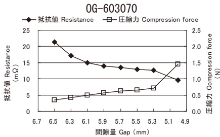
圧縮抵抗特性データ/Compression force vs Electric resistance
